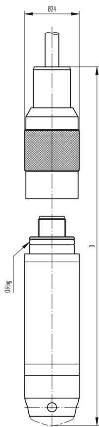
Fig. 4 Electrical connection, connectable
